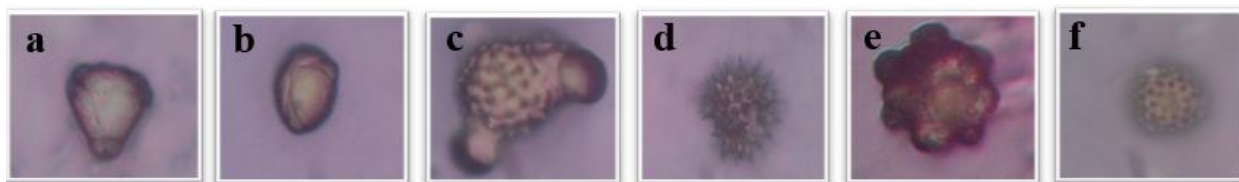
Figure 1 Melissopalynological analysis of thistle honey (400x the total magnification). a) Porter weeds sp., b) Cynara sp., c) Cotton thistles sp., d) Cirsium vulgare, e) Silybum marianum and f) Galactites sp..
