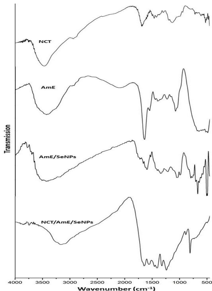
Figure 2 The produced selenium nanoparticles with Amla extract (AmE/SeNPs), their nanocomposites with nano-chitosan (AmE/Se/NCT), and the plain chitosan nanoparticles (NCT) and Amla extract (AmE) FTIR spectra.
