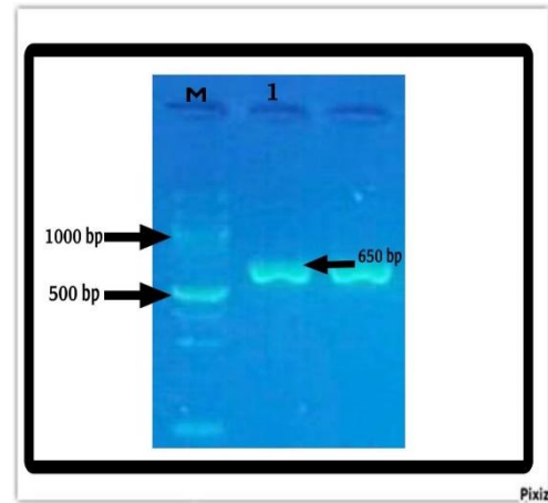
Figure 2 DNA amplification of the fungal isolate on agarose gel Path M represents: size marker, 1-2 DNA amplification of fungal isolate
