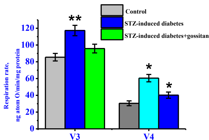
Figure 2 The effect of gossitan on mitochondrial respiration in states V_3 and V_4 with succinate of the rat liver mitochondria in the STZ-induced diabetes condition. * P < 0,05 ; ** P < 0,01 ; n = 6 .
