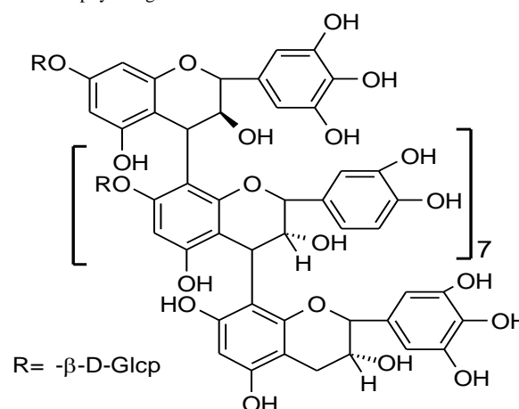
Figure 1 Chemical structure of gossitan
