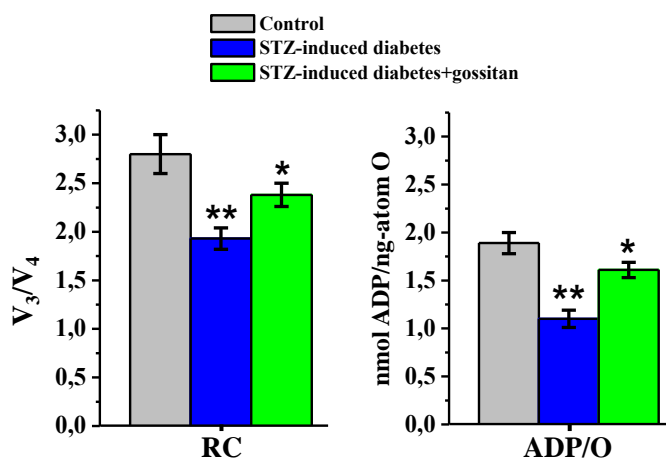
Figure 3 The influence of gossitan on respiration control and ADP/O ratio in the rat liver mitochondria of with STZ-induced diabetes. * P < 0,05 ; ** P < 0,01 ; n = 5 .
