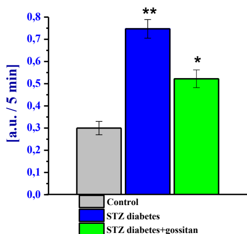
Figure 4 Changes in the swelling of rat liver mitochondria under conditions of STZ-induced diabetes and during pharmacotherapy with gossitan. The incubation medium: sucrose - 200 mM, \text{KH}_2\text{PO}_4 - 1 mM, succinate - 5 mM, \text{Ca}^{2+} -EGTA-buffer 20 - \mu\text{M} , HEPES - 20 mM, Tris-HCl - 20 mM, rotenone - 2 \mu\text{M} , oligomycin - 1 \mu\text{g}/\text{ml} , pH 7.2 (* - P < 0.05 ; ** - P < 0.01 ; n = 5).
