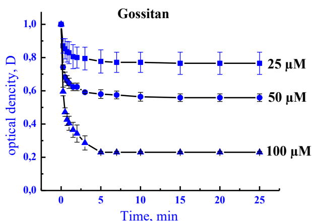
Figure 1 The change in the relative optical density of a solution of DPPH in ethanol with the addition of gossitan. The concentration of a pair of charmed mesons is 0.1 mM.
