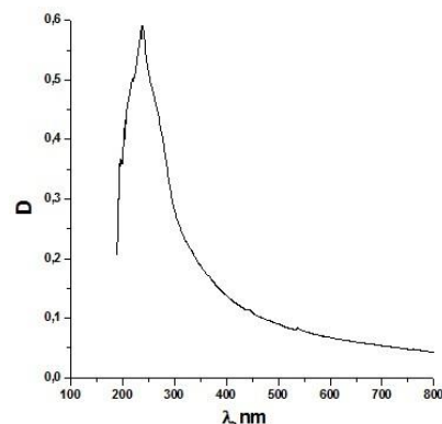
Figure 4 UV-Vis spectrum of the cellular biopolymer of R. erythropolis Au-1 strain.
