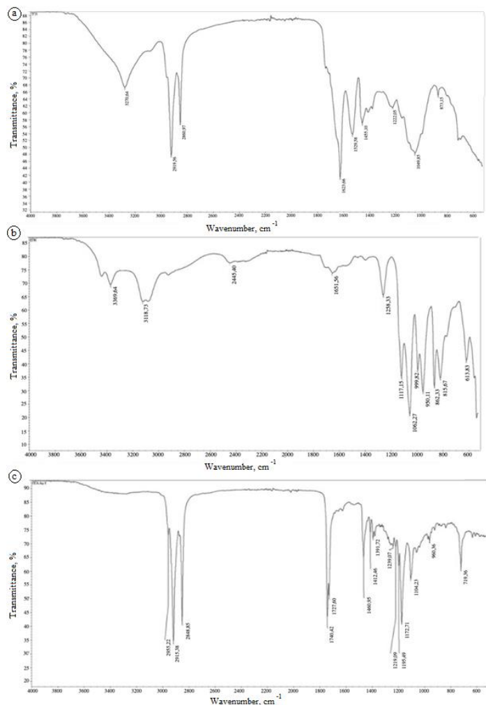
Figure 3 IR spectrums of metabolites of R. erythropolis Au-1: (a) trehalose-6,6'-dimycolate (fraction № 3 of trehalose lipid surfactants), (b) exopolysaccharide, (c) the cellular biopolymer
