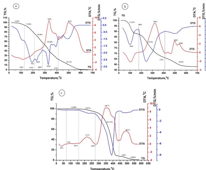
Figure 6 Thermogram of metabolites of R. erythropolis Au-1 strain: (a) trehalose-6,6'-dimycolate, (b) exopolysaccharide, (c) the cellular biopolymer; TG – thermogravimetric curve; DTA – differential thermal analysis curve; DTG – differential thermogravimetric curve.
