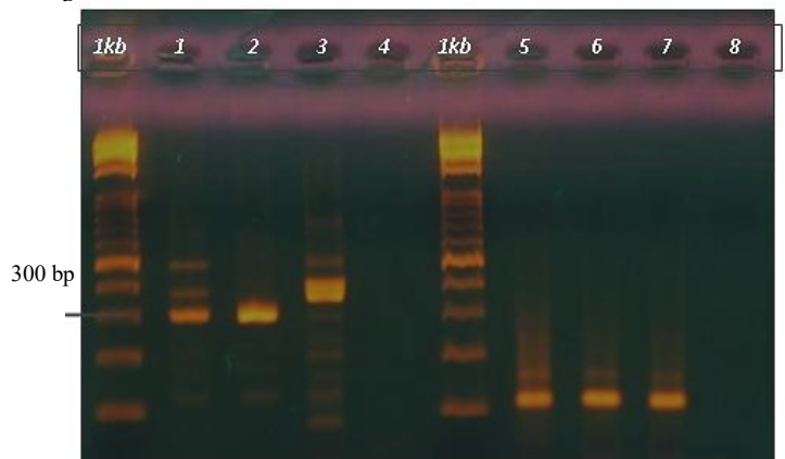
Figure 1 Gel electrophoresis of PCR products from amplification of trnH-psbA : Ladder100 bp DNA Marker, Samples 1: Brassica spp. B1, 2: Brassica spp. B2, 3: canola, 4: negative control, Ladder100 bp DNA Marker, 5: 18SrRNA B1, 6: 18SrRNA B2, 7: positive control, 8: minus template (water) control 18srRNA. PCR products were resolved on 1% TAE agarose gel
