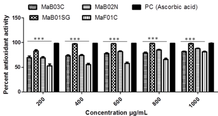
Figure 1 Percentage of antioxidant activity of selected endophytic extracts. These results are representative of the antioxidant experiment in triplicates with mean ± SEM. Statistical significance against Ascorbic acid as positive control; ***P < 0.001. (***) denotes significant value
