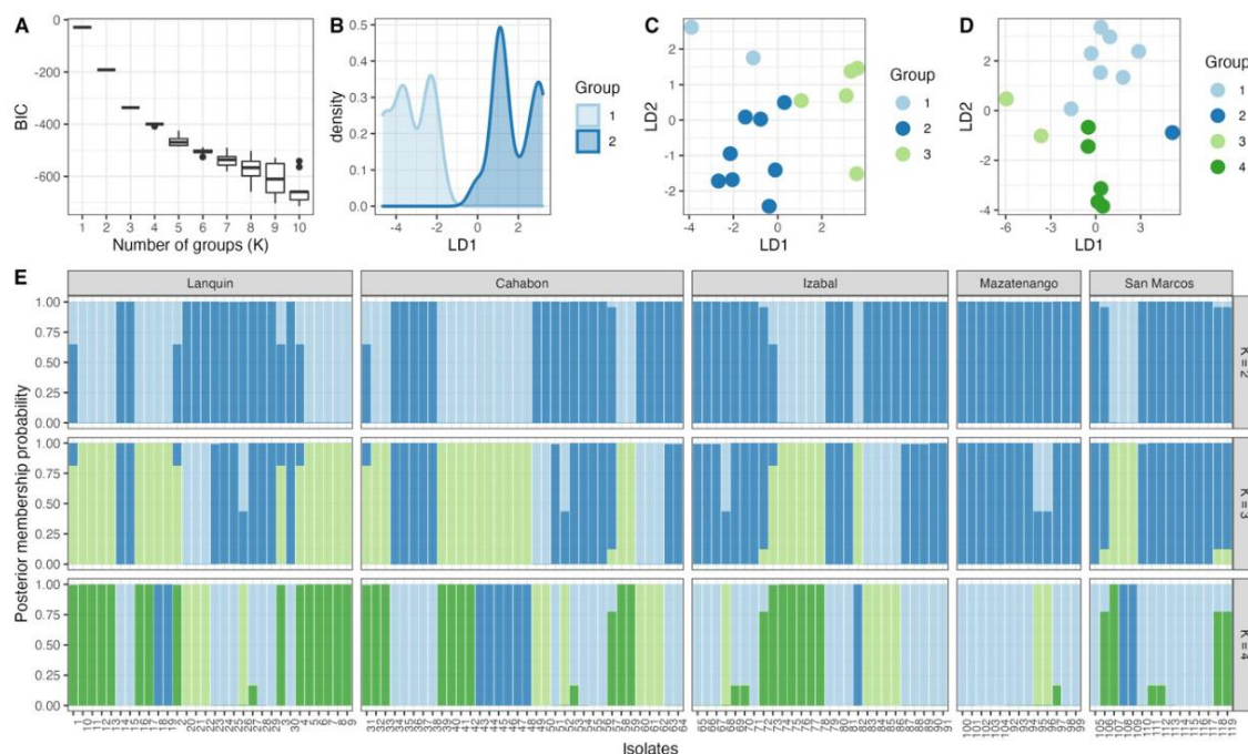
Figure 5. A) Bayesian Information Criterion value for a range of clusters (K) allowed inference of the most likely number of clusters K = 3 based on the elbow method. B) DAPC density plot of the 119 isolates against the first discriminant function retained. C) and D) DAPC scatter plot of the 119 isolates grouped in 3 and 4 cluster, respectively. E) A barplot representation of DAPC results with K means groups used as priors. The assignment probabilities of the MLG to groups identified by the cluster analysis is presented in a STRUCTURE-like form with different colors representing the cluster. Assignment probabilities to K = 2, K = 3 and K = 4 are displayed.
