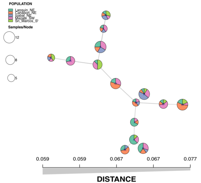
Figure 4 Minimum spanning network (MSN) constructed using Nei's distance from AFLP data set of 15 multilocus genotypes of Moniliophthora roreri . The sizes of the nodes are proportional to the number of isolates representing the MLG and the thickness of the lines represent the Nei's genetic distance between two nodes (thicker lines denote smaller genetic distance).
