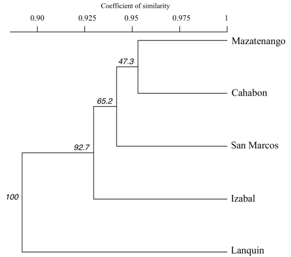
Figure 3 UPGMA dendrogram based on Nei's distance from AFLP data set of populations of Moniliophthora roreri from different cocoa producing areas in Guatemala. Values at the nodes of the branches represent bootstrap values out of 1,000 iterations.
