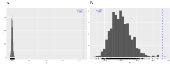
Figure 2 Standardized index of association, \bar{r}_d as the measure of linkage disequilibrium (LD) for A) complete dataset and B) unique haplotypes (clone corrected data). The observed \bar{r}_d falls outside of the distribution expected under free recombination (dotted blue line). p < 0.01 indicates significant LD (at 99.9% level).
