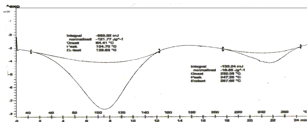
Figure 5 (b) DSC of ZnO nanoparticles loaded sago starch film
