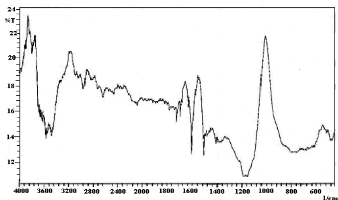
Figure 1 a) FTIR of Plain sago starch film
