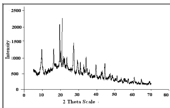
Figure 3 XRD of ZnO nanoparticles loaded sago starch film
