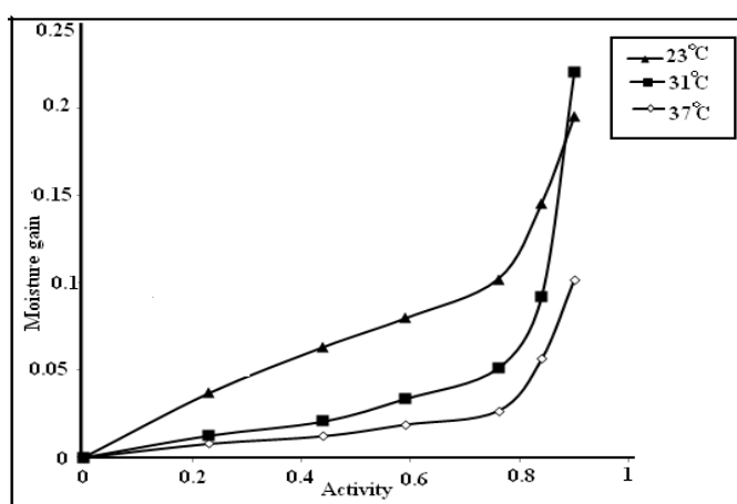
Figure 6 (b) Moisture sorption isotherm of Zinc oxide nano particles loaded sago starch film
