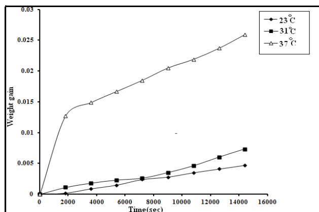
Figure7b) Kinetics of water vapor transmission through ZONLSS film.
