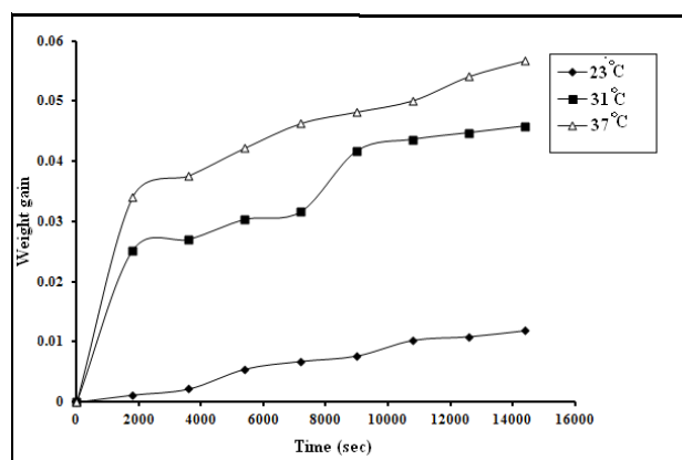
Fig 7a) Kinetics of water vapor transmission through PSS film.
