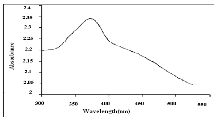
Figure 2 Surface Plasmon Spectrum for ZnO nanoparticles
