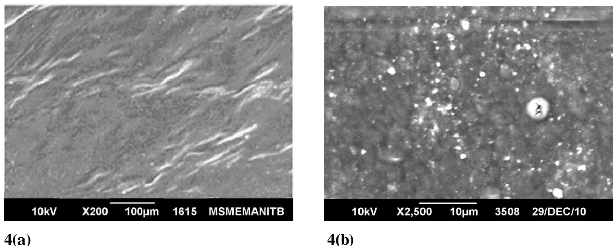
Figure 4 (a) SEM image of Plain sago starch film, (b) SEM image of ZnO nano particles loaded sago starch film
