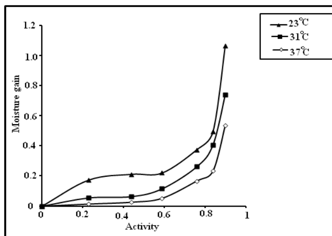
Figure 6 (a) Moisture sorption isotherm of Plain sago starch film
