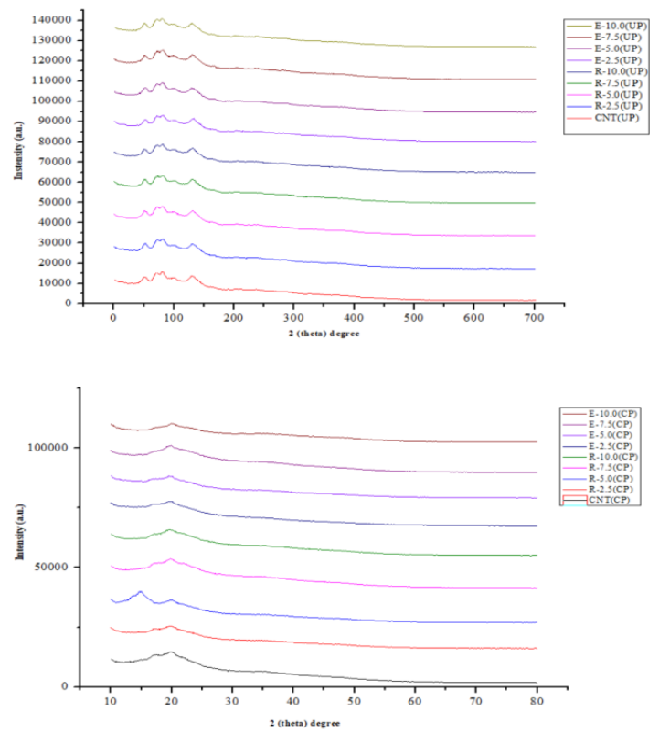
Figure 2 X-ray diffraction pattern of uncooked and cooked Pasta samples
