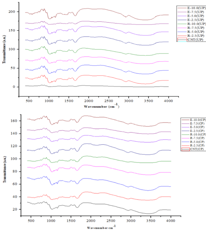
Figure 1 FTIR spectra of the uncooked and cooked pasta samples
